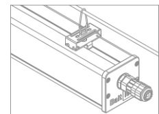
Stainless-steel surface/rope mounting kit BWL-SRKITZ
